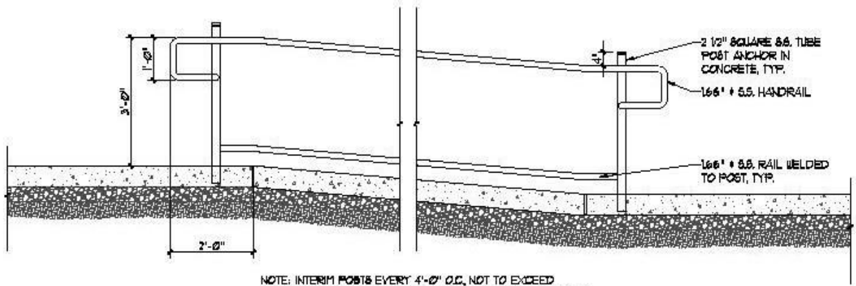
SECTION - HANDRAIL AT RAMP
